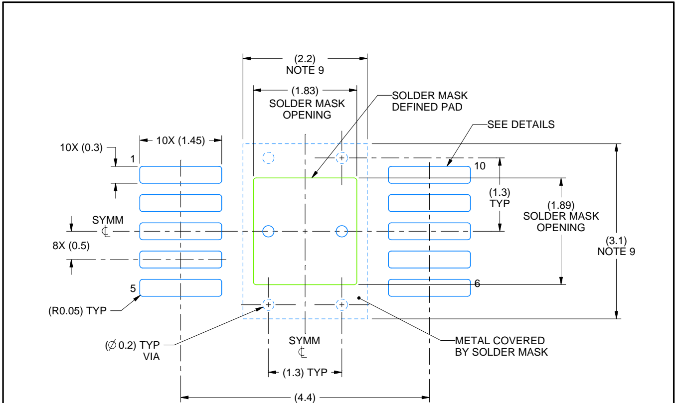
LAND PATTERN EXAMPLE SCALE:15X
